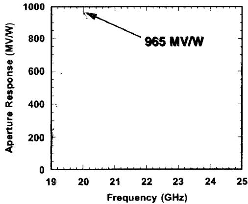
Fig. 6. The measured system video responsivity versus frequency. The 3-dB bandwidth is 1500 MHz.
