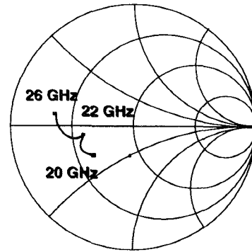
Fig. 3. The measured input impedance of the double folded-slot antenna design shown in Fig. 2.
