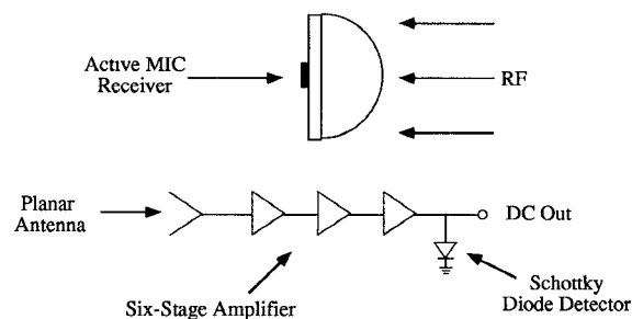
Fig. 1. Layout of the uniplanar active receiver/radiometer with a double-folded slot antenna and silicon substrate lens.
