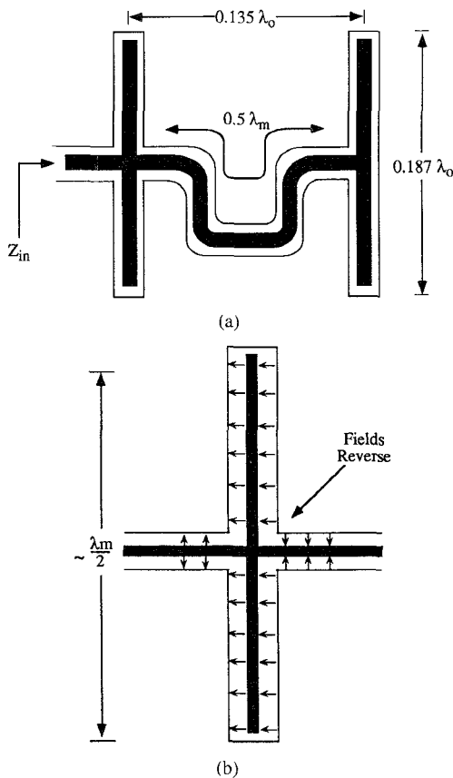
Fig. 2. The double folded-slot antenna design on a (a) GaAs half-space and (b) the field distribution around a folded-slot antenna.
