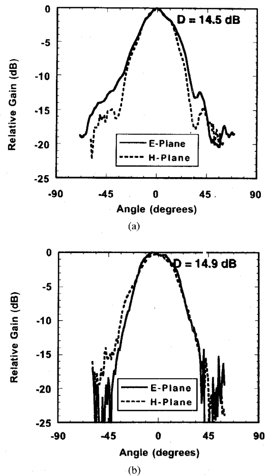
Fig. 5. The measured far-field patterns at (a) 20 and (b) 22 GHz. The silicon substrate lens is 2.54 cm in diameter.
